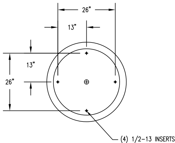
3 BOTTOM VIEW
