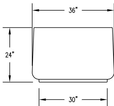
2 ELEVATION VIEW
