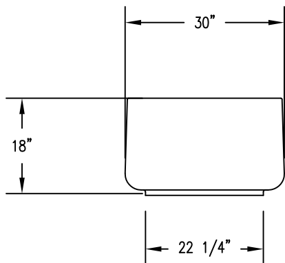
2 ELEVATION VIEW
