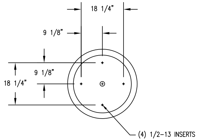
3 BOTTOM VIEW
