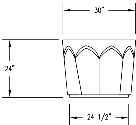
2 ELEVATION VIEW
