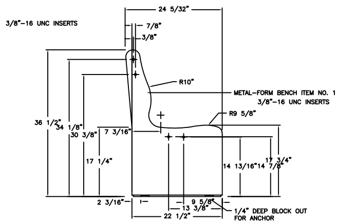
SIDE VIEW BENCH LEG
