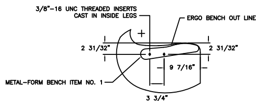
DETAIL BOLT LOCATION BENCH
