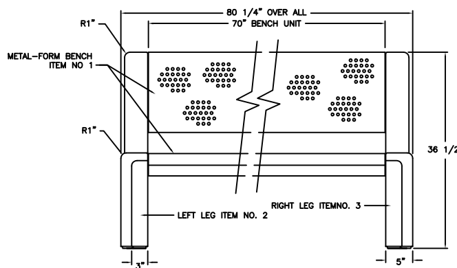
FRONT ELEVATION SET
