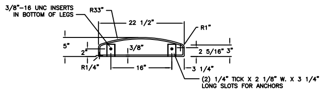
BOTTOM VIEW BENCH LEG
