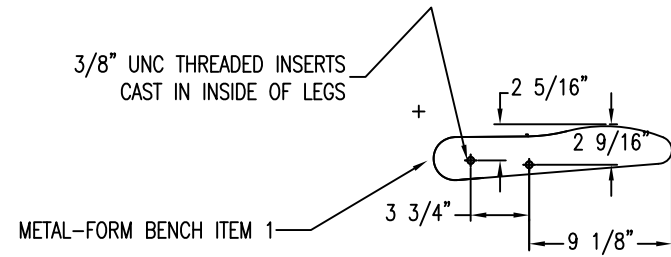
DETAIL BOLT LOCATION BENCH
