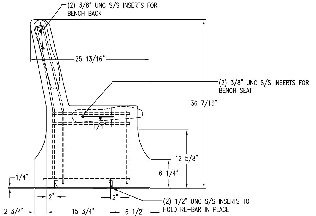
INSIDE ELEVATION BENCH ENDS
