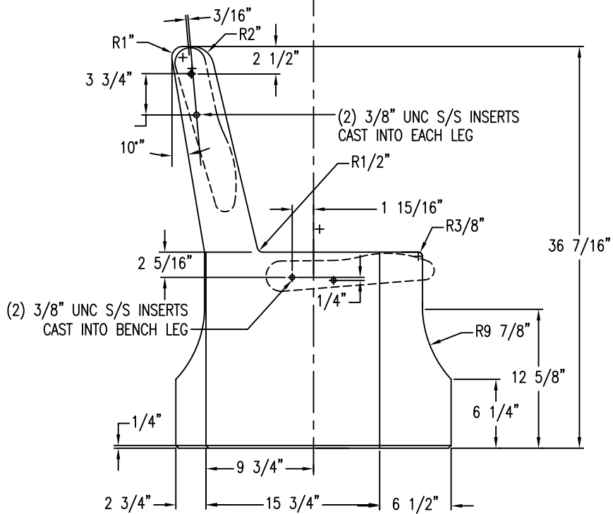
INSIDE ELEVATION BENCH ENDS
