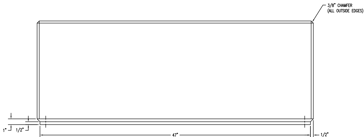
ELEVATION VIEW
