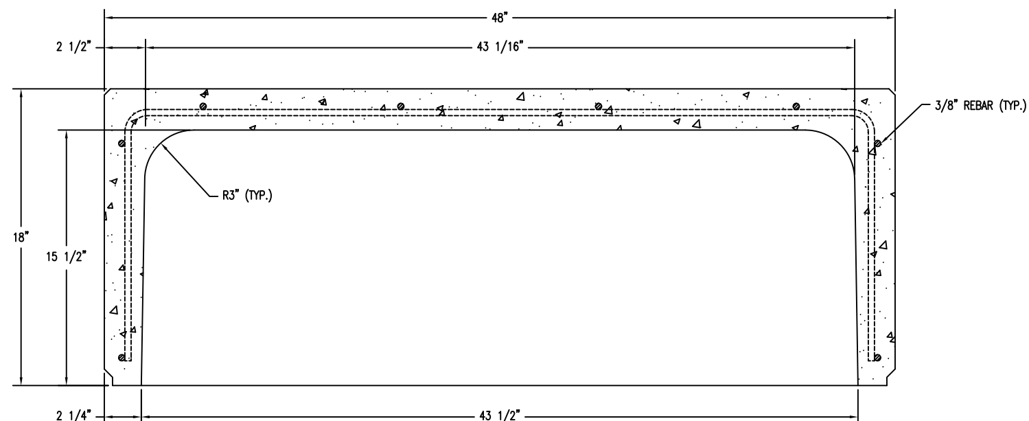
SECTION VIEW
