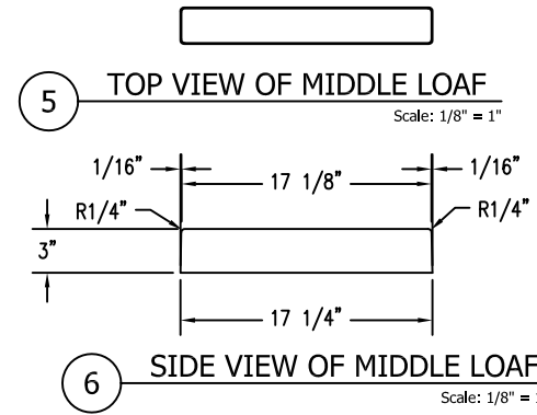
6 SIDE VIEW OF MIDDLE LOAF Scale: 1/8" = 1"
