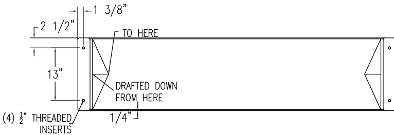
3 BOTTOM VIEW Scale: 1/16" = 1"
