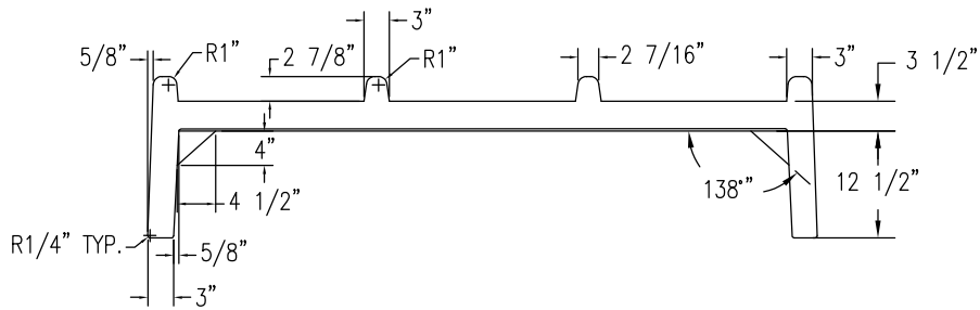
2 ELEVATION VIEW Scale: 1/16" = 1"
