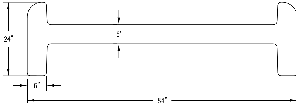
SIDE ELEVATION CAST CONCRETE BENCH
