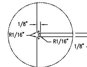
A ENLARGED DETAIL OF REVEAL LINE Scale: 1" = 1"
