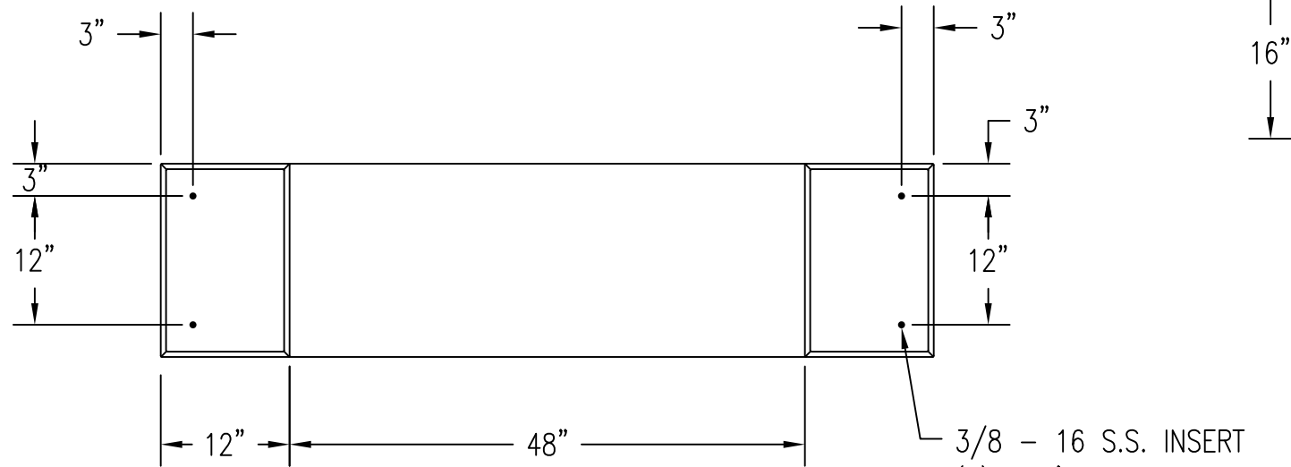
3 BOTTOM VIEW OF BENCH Scale: 1/16" = 1"
