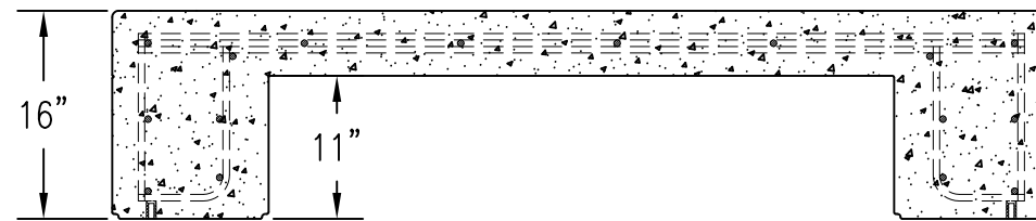
5 SECTION VIEW OF BENCH Scale: 1/16" = 1"
