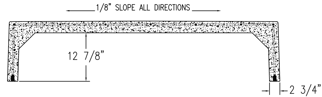
5 SECTION VIEW Scale: 1/16" = 1"
