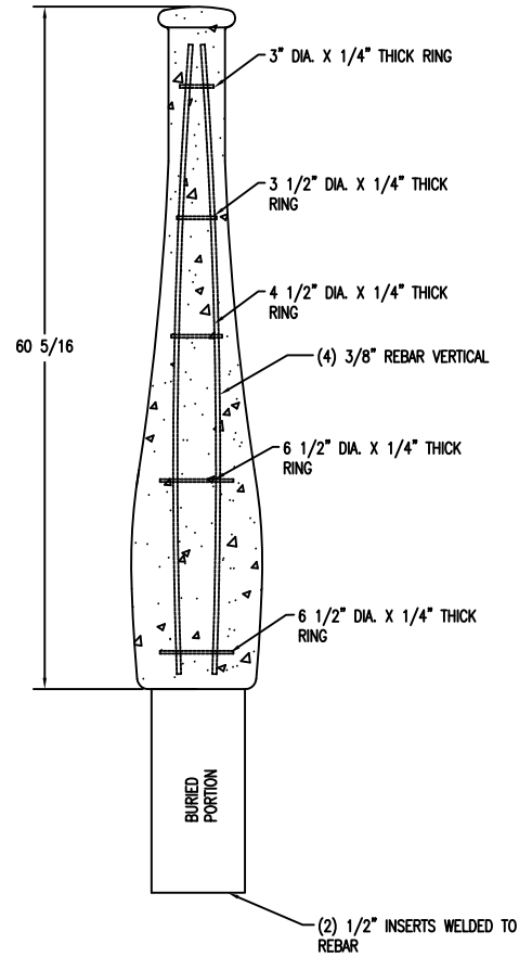
3 SECTION VIEW OF BOLLARD Scale: NTS
