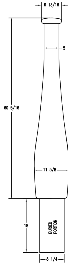
1 ELEVATION VIEW OF BOLLARD Scale: NTS
