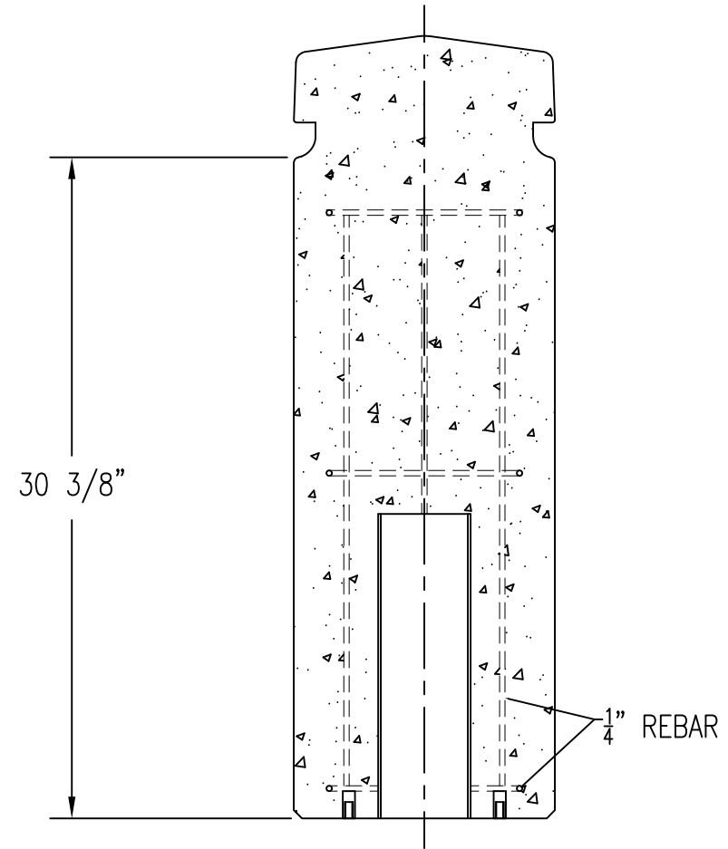
4 CROSS SECTION
