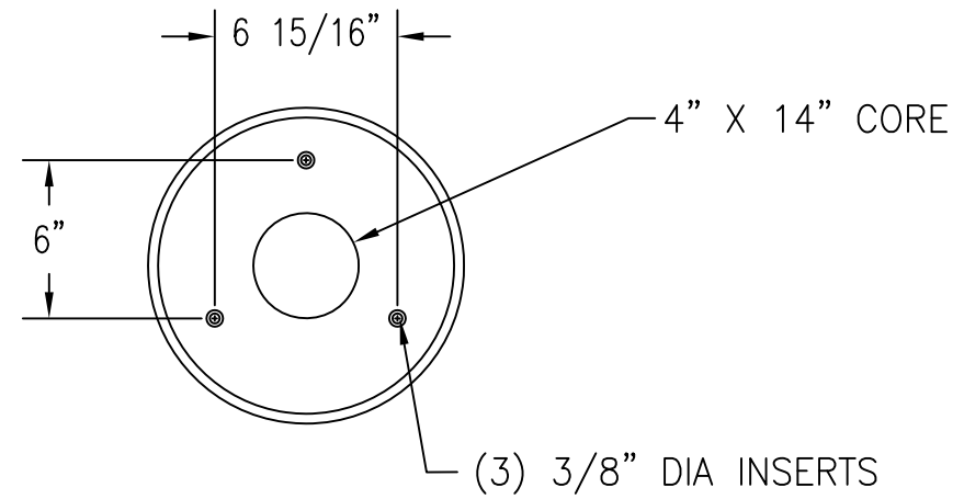
3 BOTTOM VIEW
