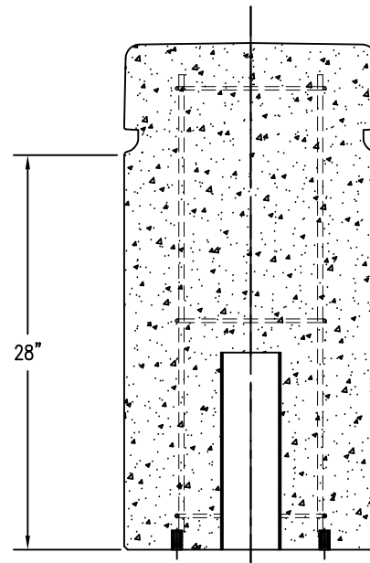
4 CROSS SECTION
