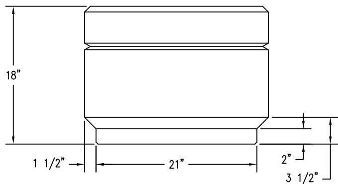
2 ELEVATION VIEW
