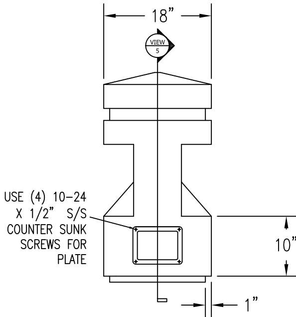
1 SIDE ELEVATION VIEW
