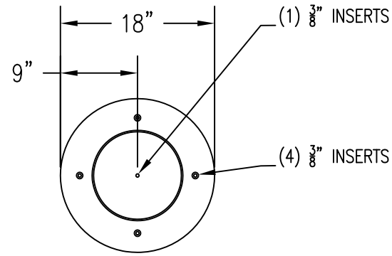
8 BOTTOM VIEW OF CAP
