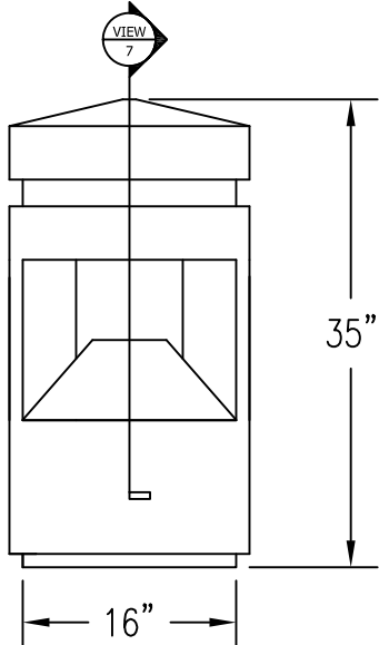
3 FRONT ELEVATION VIEW
