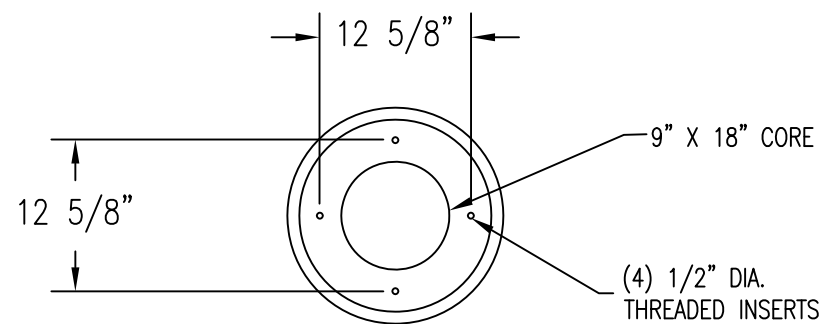
4 BOTTOM VIEW
