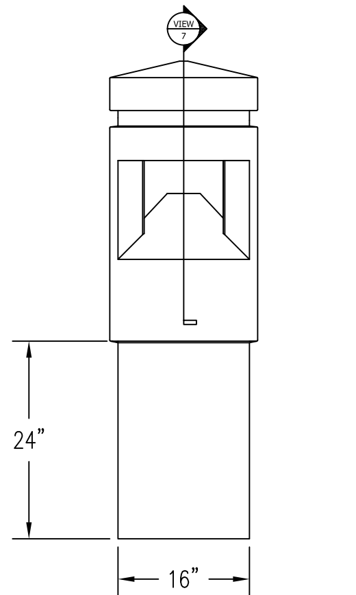
3 FRONT ELEVATION VIEW
