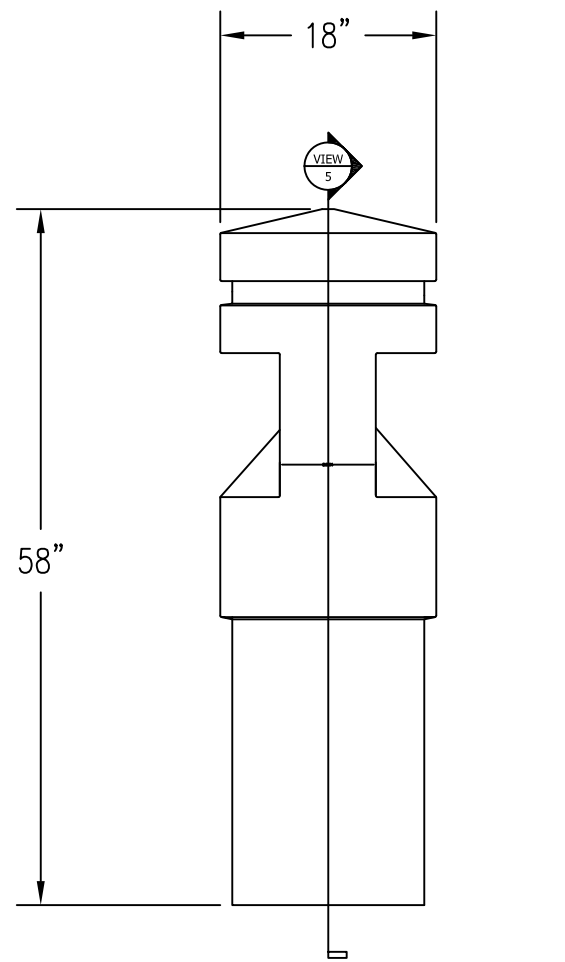
1 SIDE ELEVATION VIEW
