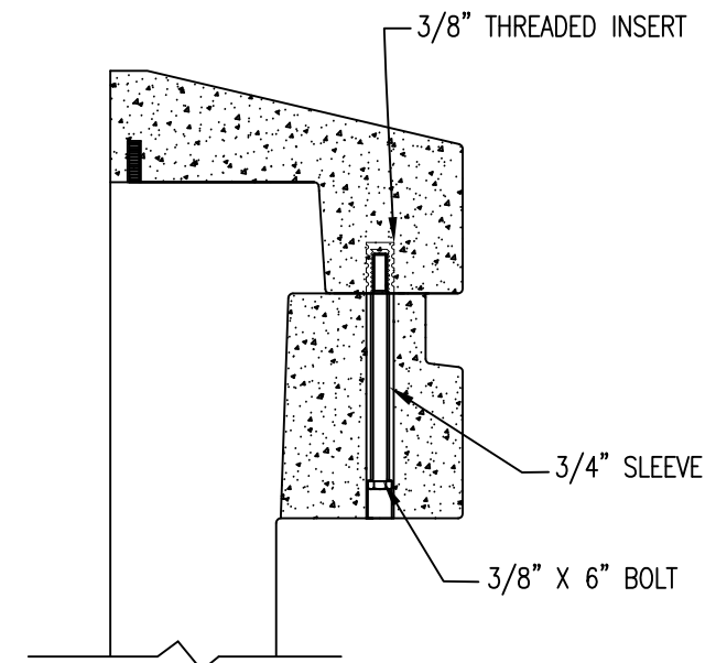
6 DETAIL
