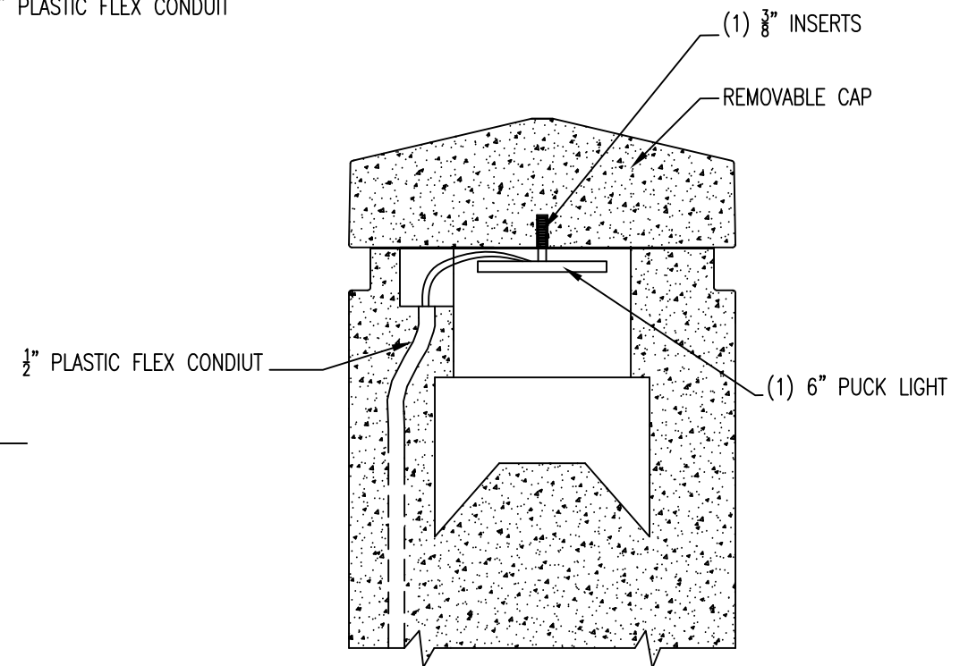
7 SECTION
