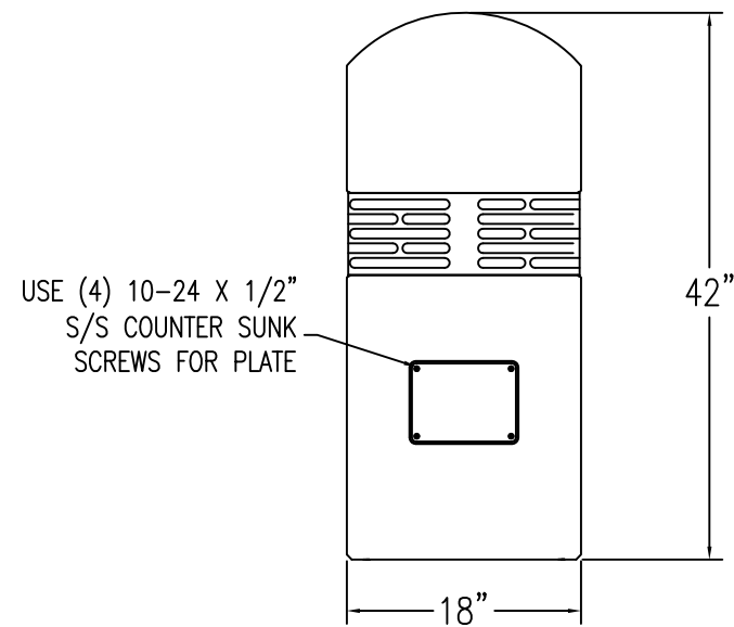
2 ELEVATION VIEW
