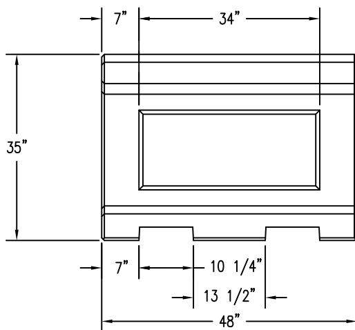
2 ELEVATION VIEW
