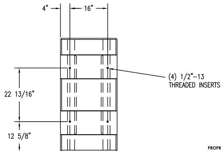
4 CROSS SECTION
