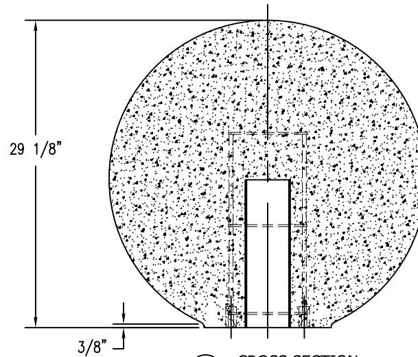
4 CROSS SECTION
