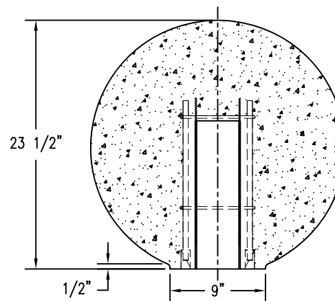
4 CROSS SECTION
