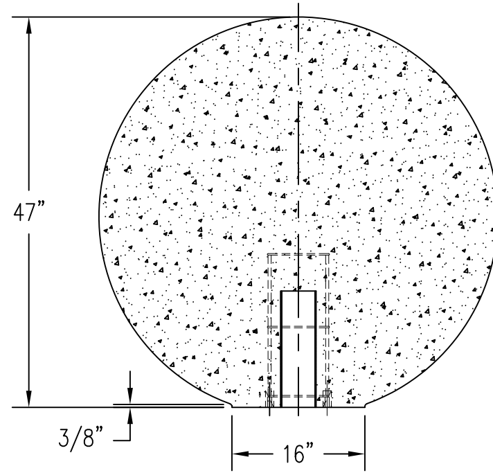
4 CROSS SECTION
