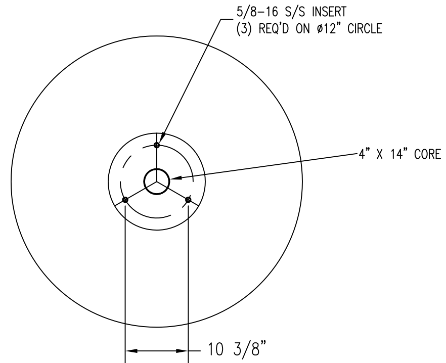
3 BOTTOM VIEW
