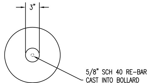
3 BOTTOM VIEW
