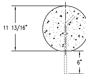
4 CROSS SECTION
