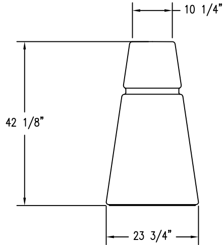
2 ELEVATION VIEW
