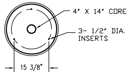
3 BOTTOM VIEW
