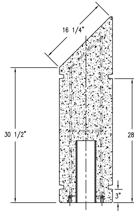
2 CROSS SECTION
