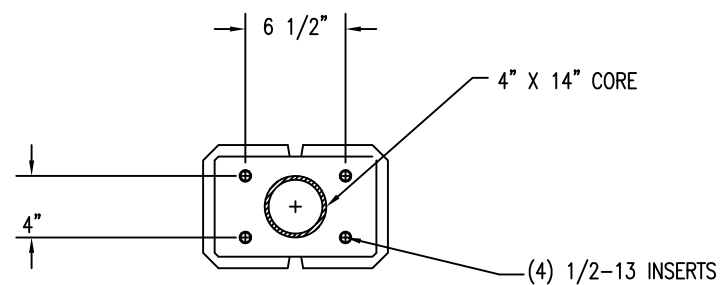
4 CROSS SECTION
