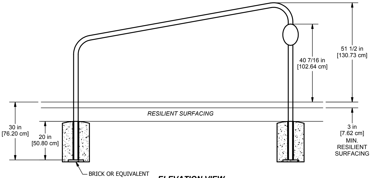
ELEVATION VIEW
