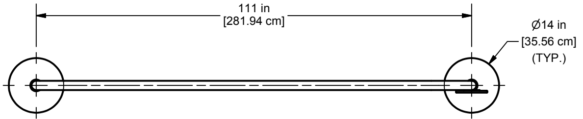
PLAN VIEW
