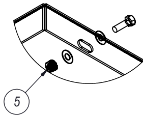
DETAIL C SCALE 1 : 5
