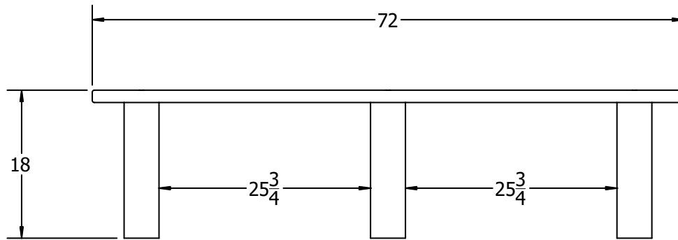
FRONT VIEW
