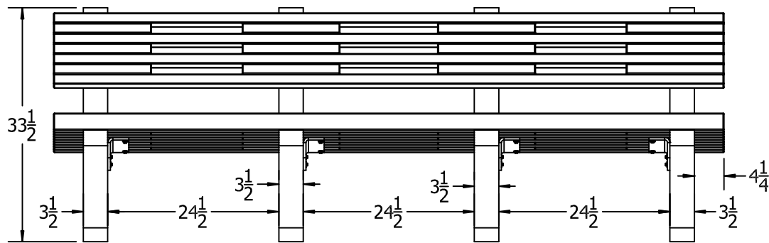
FRONT VIEW
